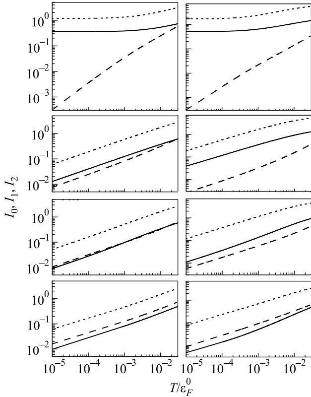
Fig.3. The transport integrals I_0 (solid lines), I_1 (dashed lines) and I_2 (short-dashed lines) in log-log scale as functions of reduced temperature T/\epsilon_F^0 , calculated with the interaction function (16) for \beta p_F = 3 (left column) and \beta p_F = 30 (right column) and four values of the parameter g corresponding to FL (upper panels), the QCP (second line of panels), and to the states with 10% (third line) and 50% (lower panels) of quasiparticles in the FC
