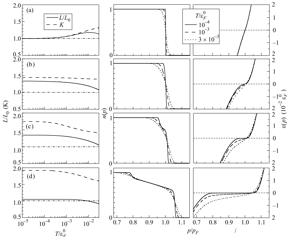
Fig.2. Same as in Fig.1 calculated with the interaction function (16) for \beta p_F = 3 and four values of the parameter g in units of M^{-1} : 3.0 (Fermi liquid, panels (a)), 3.55 (QCP, panels (b)), 3.9 (the state with the FC fraction \rho_{FC}/\rho = 0.1 panels (c)), and 4.8 (the state with \rho_{FC}/\rho = 0.5 , panels (d))
