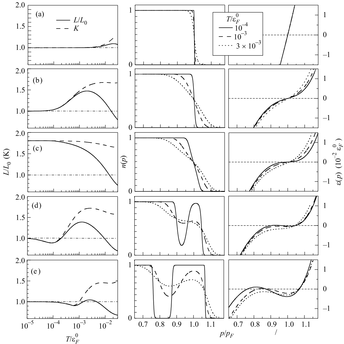
Fig.1. The reduced Lorenz number L(T)/L_0 together with the ratio K(T) = 3I_2(T)/\pi^2 I_0(T) (left panels) as functions of the reduced temperature T/\epsilon_F^0 , the occupation numbers n(p) (middle panels) and the single-particle spectrum (right panels) calculated at different line-type-coded temperatures with the interaction function (14) for five different sets of input parameters, which correspond to five different cases: Fermi liquid with the effective mass M^*/M \simeq 6 , i.e. quite far from the QCP (panels (a)); Fermi liquid with M^*/M \simeq 80 , which is close to the QCP (panels (b)); system at the QCP (panels (c)), the state just beyond the QCP, with p_2 - p_1 \simeq 0.14 p_F (panels (d)) and the state well beyond the QCP, with p_2 - p_1 \simeq 0.31 p_F (panels (e))
