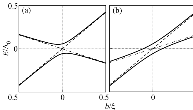
Fig. 1. Shown by solid lines is the spectrum transformation caused by the interaction of vortex and surface spectrum branches: (a) chirality and vorticity have different signs ( \eta = 1, \chi = -1 ); (b) chirality and vorticity have the same signs ( \eta = 1, \chi = 1 ). The dash and dash-dotted curves correspond to the non-interacting vortex and surface energy branches
