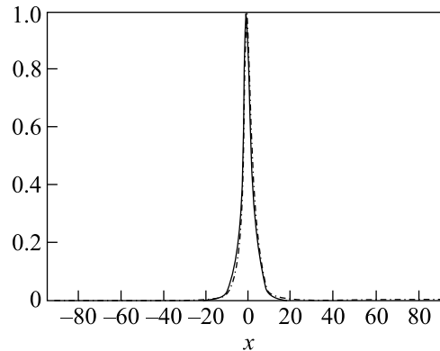
Fig.2. Initial (solid line) and final (dashed line) at t = 2.7192 distributions for |\bar{\psi}| , WW solitons, self-similar variables. The soliton amplitude was increased by 1%, \mu = 1 , \lambda = 1 . The ratio between final and initial soliton amplitudes in the physical variables is about 11
