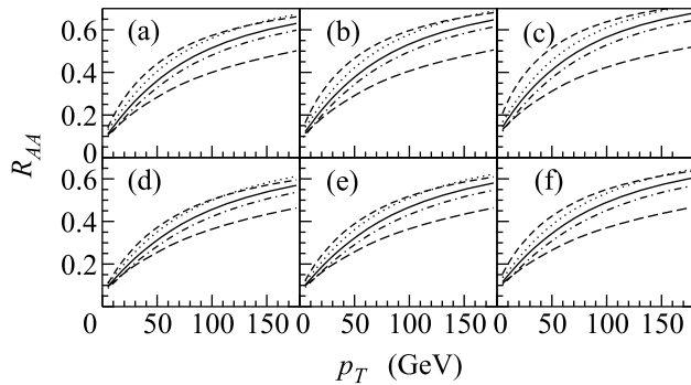
Fig.3. The same as in Fig.1 for Pb+Pb collisions at \sqrt{s} = 5500 GeV
