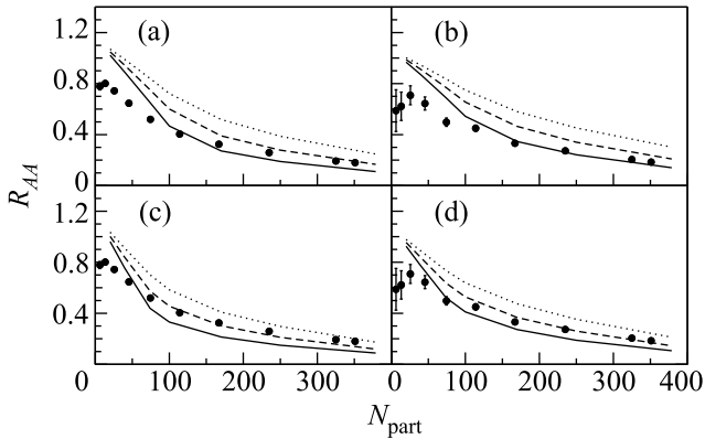
Fig.2. The nuclear modification factor R_{AA} for \pi^0 production in Au+Au at \sqrt{s} = 200 GeV for p_T > 5 GeV (left panels) and p_T > 10 GeV (right panels) as a function of N_{\text{part}} . The upper panels are for the chemically equilibrium plasma, and the lower ones for purely gluonic plasma with the same entropy. The theoretical curves show the total (quarks plus gluons) R_{AA} including the radiative plus collisional energy loss and the energy gain due to gluon absorption for \alpha_s^{fr} = 0.7 (solid line), \alpha_s^{fr} = 0.5 (dashed line), \alpha_s^{fr} = 0.7 (dotted line). The experimental points are from [16]
