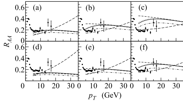
Fig.1. The nuclear modification factor R_{AA} for \pi^0 production in the central Au+Au collisions at \sqrt{s} = 200 GeV for \alpha_s^{f_r} = 0.7 ((a),(d)), \alpha_s^{f_r} = 0.5 ((b),(e)), \alpha_s^{f_r} = 0.4 ((c),(f)). The upper panels are for the chemically equilibrium plasma, and the lower ones for purely gluonic plasma with the same entropy. For all the theoretical curves L_{\text{max}} = 8 fm. Solid line: the total (quarks plus gluons) radiative R_{AA} . Dashed line: the radiative R_{AA} for \pi^0 from quarks. Long-dash line: the radiative R_{AA} for \pi^0 from gluons. Dash-dotted line: the total (quarks plus gluons) R_{AA} including the radiative plus collisional energy loss and the energy gain due to gluon absorption. Dotted curves show the total (quarks plus gluons) radiative R_{AA} for the inverse time order of the DGLAP and induced gluon emission stages. The experimental points are the data obtained by the PHENIX Collaboration [16] for the most central (0–5%) collisions
