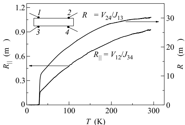
Fig.1. Temperature dependences R_{\parallel}(T) and R_{\perp}(T) . The contact positions for Montgomery measurements are shown in the insert
