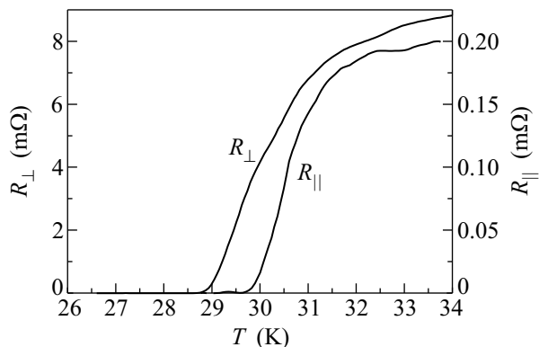
Fig.3. The influence of the current direction on the superconducting transition temperature
