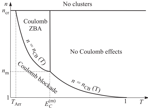
Fig.4. Different regimes for tunneling between two clusters with n grains each on the n-T plane. The most interesting case n_{\text{cr}} > n_m is shown; in the opposite case, for n_{\text{cr}} < n_m , there are no clusters in the ‘‘Coulomb ZBA’’ domain
