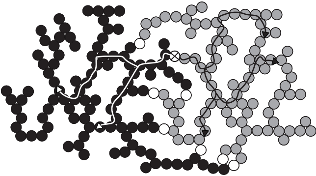
Fig.3. The charge spreading process. After the tunneling of an electron between two clusters (black and grey) through one of the links (marked by a cross) a diffusional spreading of charge occurs in both clusters
