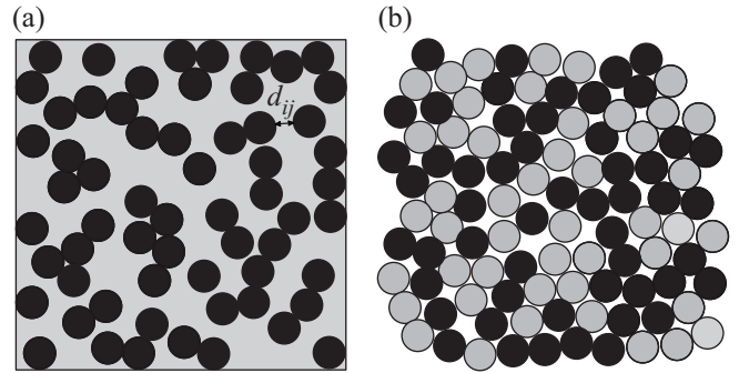
Fig.1. Clusters of conducting grains in granular materials. (a) – Metal grains (shown black) in an insulating matrix (shown grey). Randomly distributed distances d_{ij} between two non-touching conducting grains determine corresponding tunnel conductances g_{ij} . (b) – A mixture of conducting and insulating grains. The “links” (one-grain insulating bridges) between two conducting clusters are supposed to have the same conductances g_{ij} = g , while all longer bridges have g_{ij} \ll g and can be neglected
