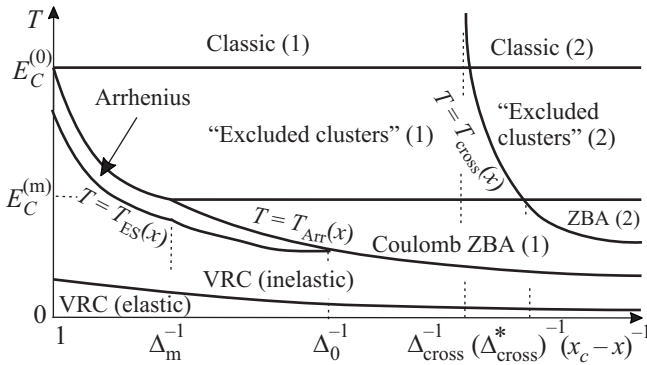
Fig.5. Phase diagram of different regimes for the conductivity. “Classic (1)” – classic T -independent transport, controlled by the links (see Eq(17)); “Classic (2)” – the same in the critical crossover region (see Eq(18)); “Excluded clusters (1)” – transport via large (non-blockaded) NNN-connected clusters, the T -dependence is a power law (see Eq.(13)); “Excluded clusters (2)” – the same in the critical crossover region (see Eq.(14)); “Coulomb ZBA (1)” – transport is controlled by the Coulomb zero-bias anomaly, the T -dependence is stretched exponential (see Eq.(28)); “ZBA (2)” – the same in the critical crossover region (see Eq.(29)); “Arrhenius” – direct hopping between Coulomb blockaded critical clusters, the T -dependence is simple activation (see Eq.(1)); “VRC” – variable range cotunneling (elastic or inelastic) between small resonant clusters via chains of critical non-resonant clusters, the T -dependence is the modified Efros-Shklovskii law (see Eq.(2))
