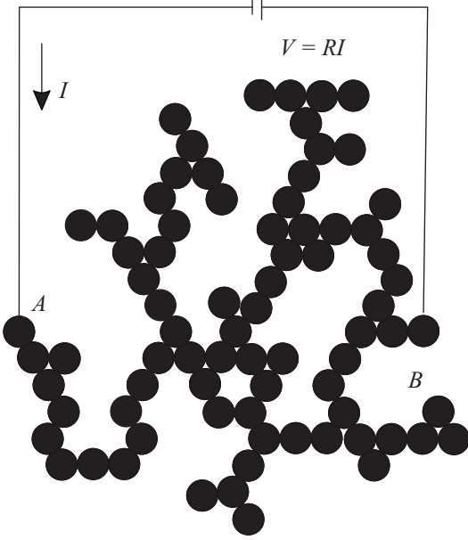
Fig.2. Definition of the classic resistance R across a cluster. External voltage V is applied to points A and B at the periphery of the cluster, then the ratio of V and the current I in the external circuit is the resistance R
